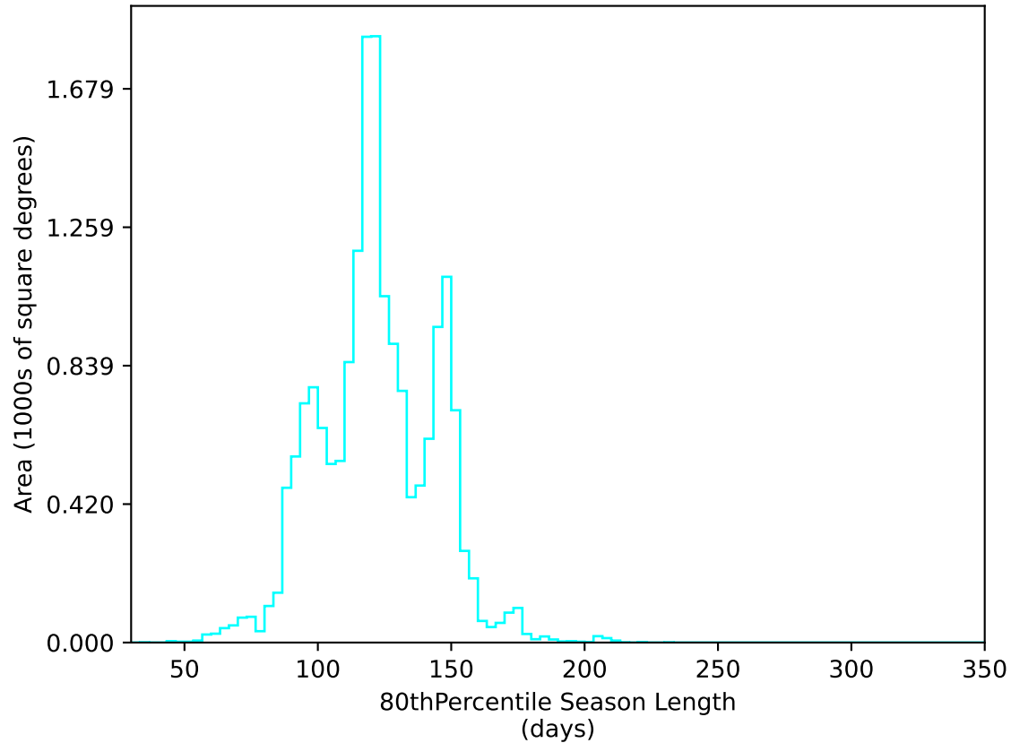
too_elab_heavy_r64_d3_gz_v3.4_10yrs WFD u band: 80thPercentile Season Length
