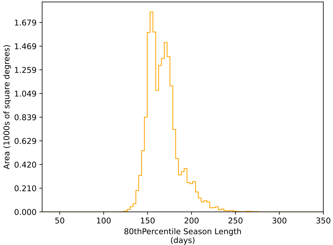
too_elab_heavy_r64_d3_gz_v3.4_10yrs WFD r band: 80thPercentile Season Length
