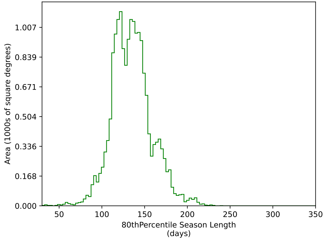
too_elab_heavy_r64_d3_gz_v3.4_10yrs WFD g band: 80thPercentile Season Length
