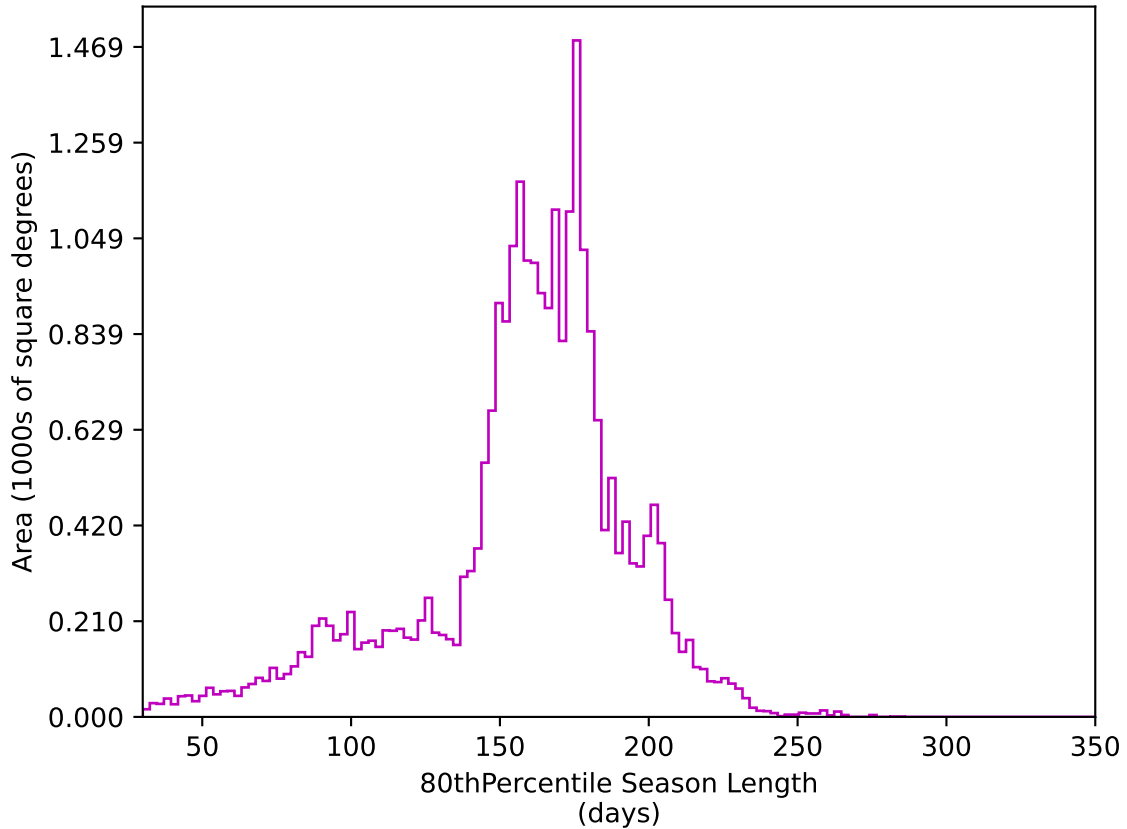
too_elab_heavy_r64_d3_gz_v3.4_10yrs All sky z band: 80thPercentile Season Length
