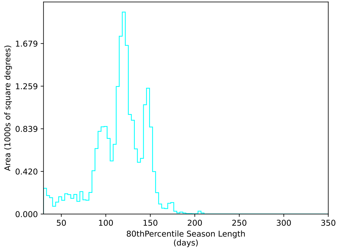
too_elab_heavy_r64_d3_gz_v3.4_10yrs All sky u band: 80thPercentile Season Length
