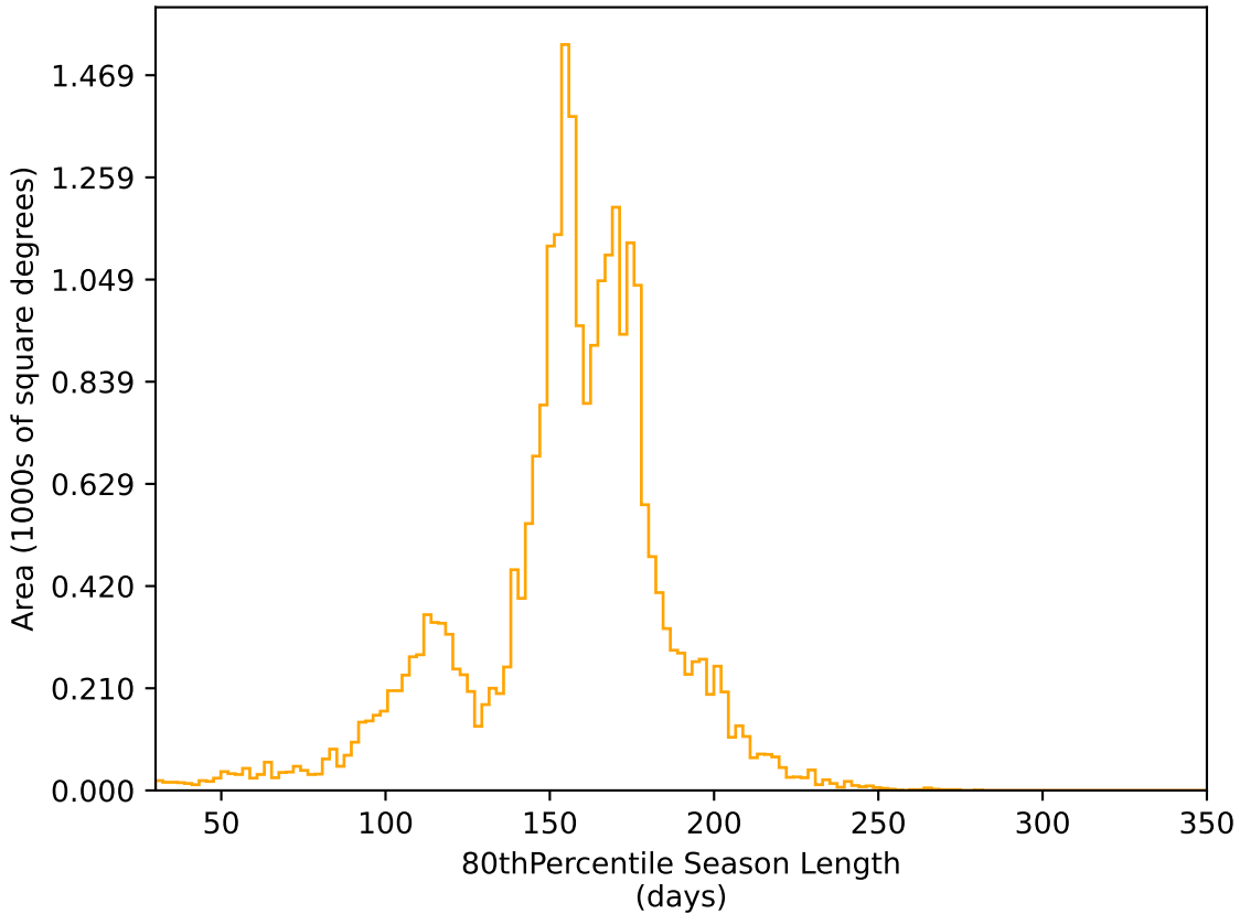
too_elab_heavy_r64_d3_gz_v3.4_10yrs All sky r band: 80thPercentile Season Length
