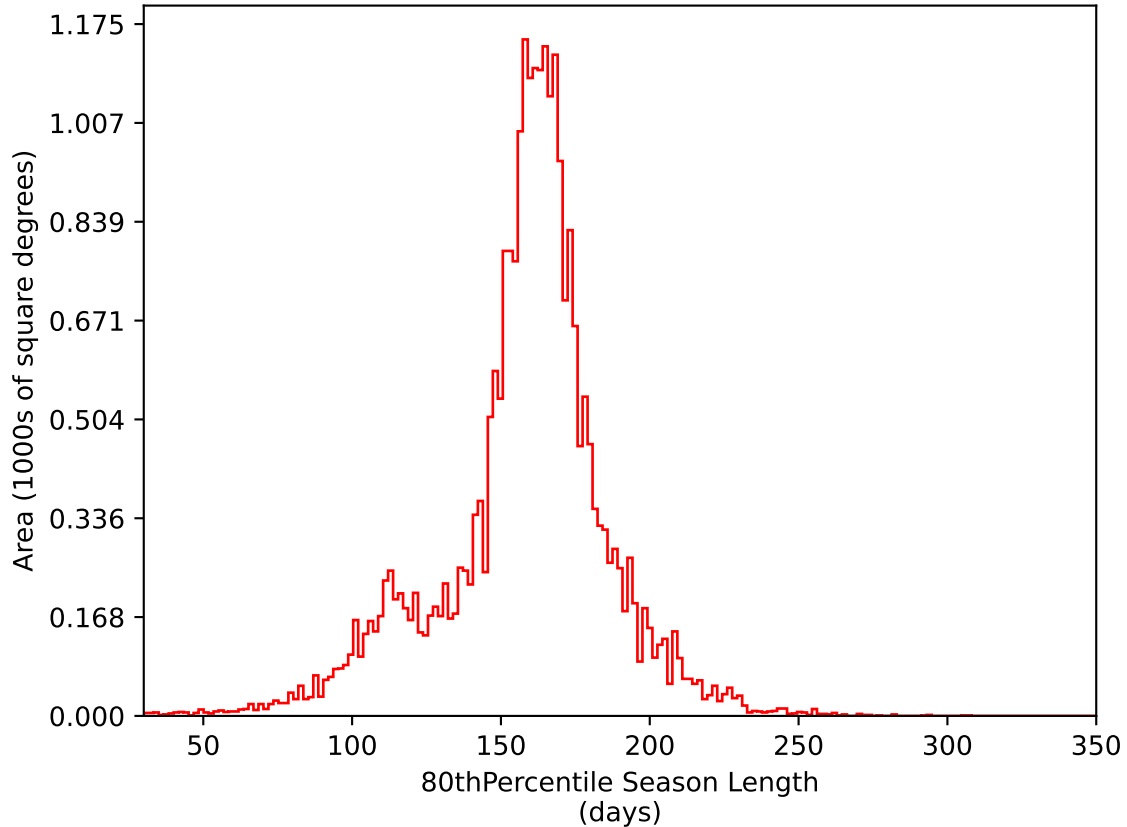
too_elab_heavy_r64_d3_gz_v3.4_10yrs All sky i band: 80thPercentile Season Length
