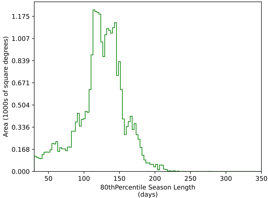
too_elab_heavy_r64_d3_gz_v3.4_10yrs All sky g band: 80thPercentile Season Length
