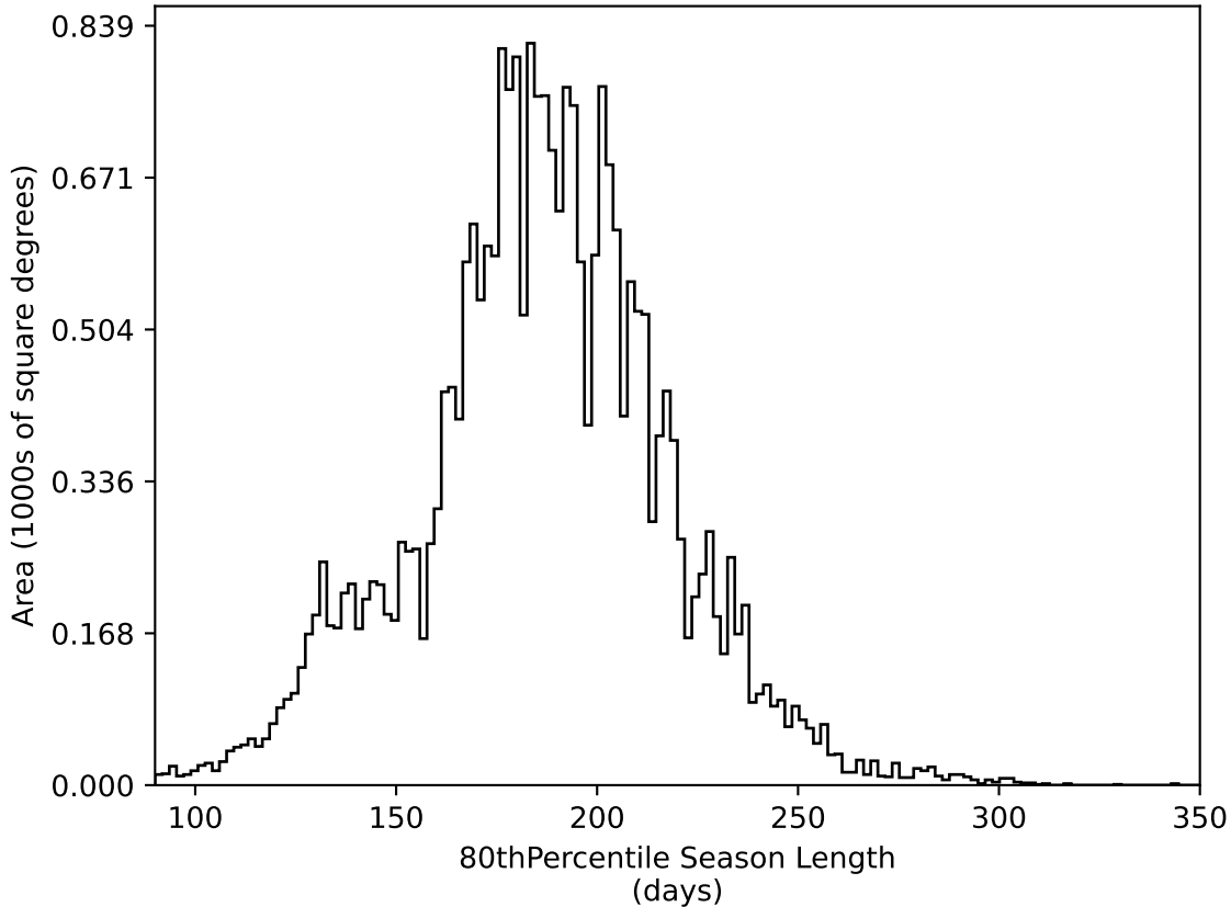
too_elab_heavy_r64_d3_gz_v3.4_10yrs All sky all bands: 80thPercentile Season Length
