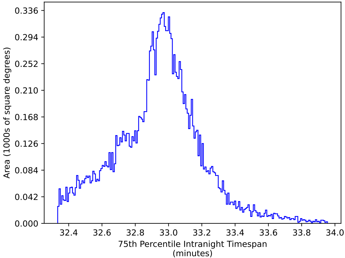
too_elab_heavy_r64_d3_gz_v3.4_10yrs WFD y band: 75th Percentile Intranight Timespan
