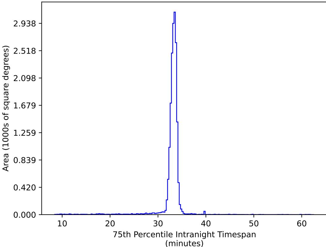
too_elab_heavy_r64_d3_gz_v3.4_10yrs WFD ug bands: 75th Percentile Intranight Timespan
