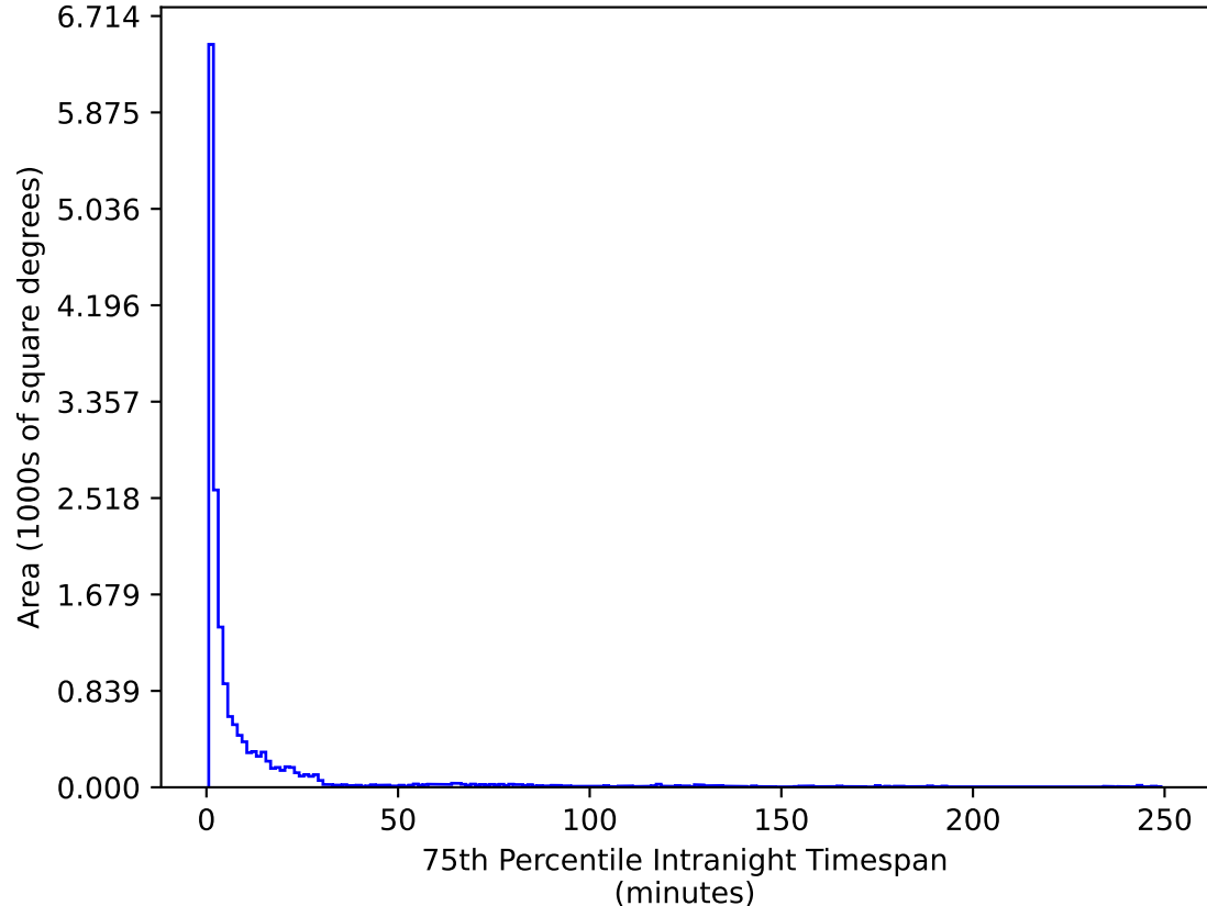
too_elab_heavy_r64_d3_gz_v3.4_10yrs WFD u band: 75th Percentile Intranight Timespan
