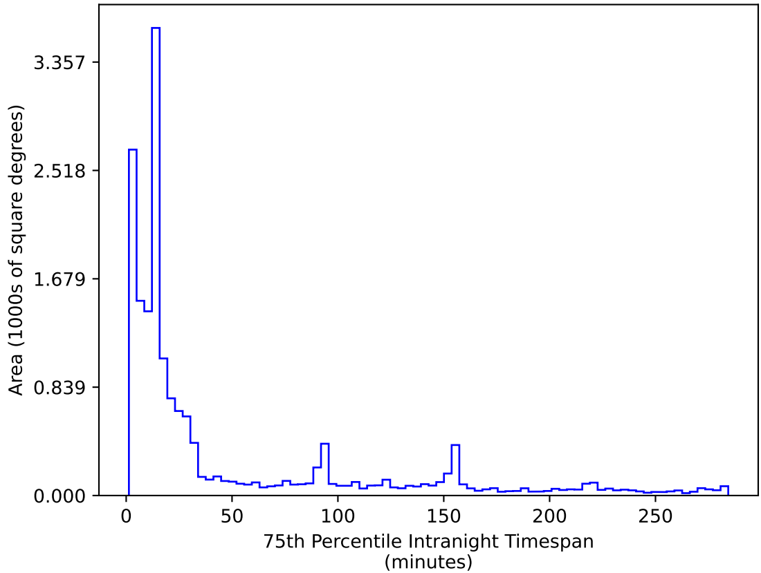
too_elab_heavy_r64_d3_gz_v3.4_10yrs WFD r band: 75th Percentile Intranight Timespan
