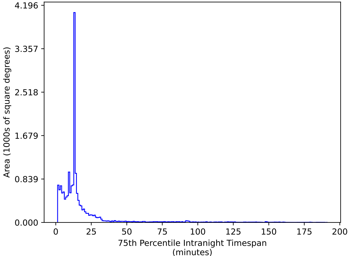
too_elab_heavy_r64_d3_gz_v3.4_10yrs WFD i band: 75th Percentile Intranight Timespan
