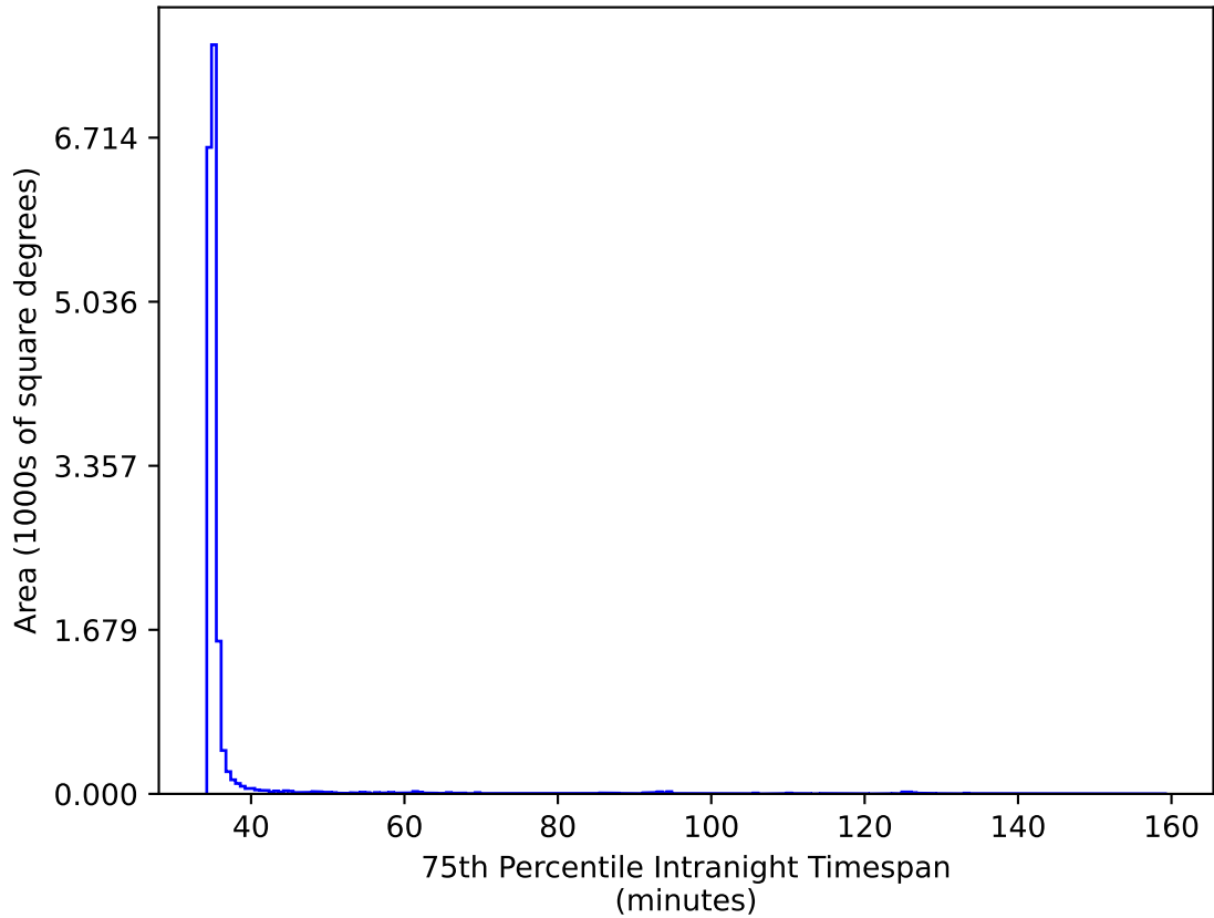
too_elab_heavy_r64_d3_gz_v3.4_10yrs WFD gr bands: 75th Percentile Intranight Timespan
