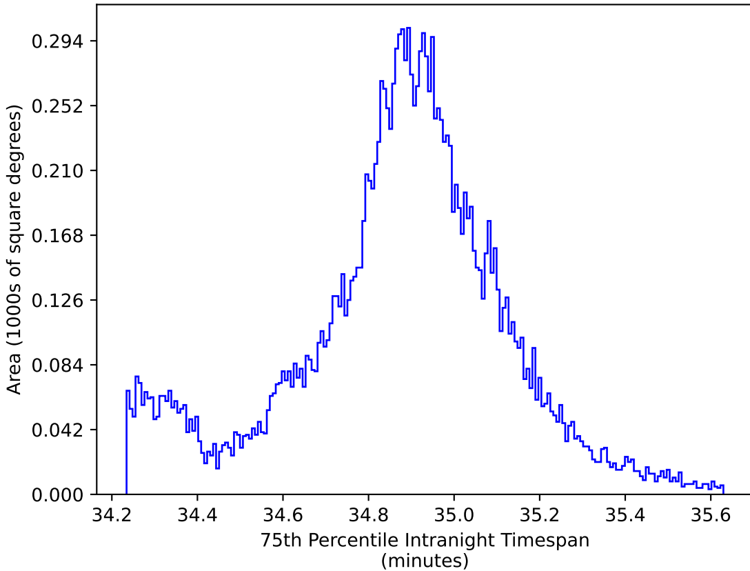
too_elab_heavy_r64_d3_gz_v3.4_10yrs WFD all bands: 75th Percentile Intranight Timespan
