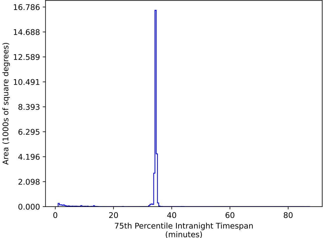
too_elab_heavy_r64_d3_gz_v3.4_10yrs All sky zy bands: 75th Percentile Intranight Timespan
