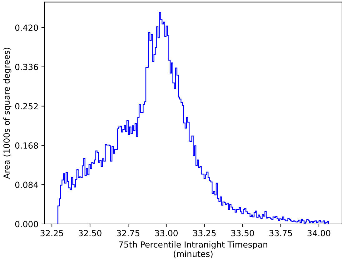
too_elab_heavy_r64_d3_gz_v3.4_10yrs All sky y band: 75th Percentile Intranight Timespan
