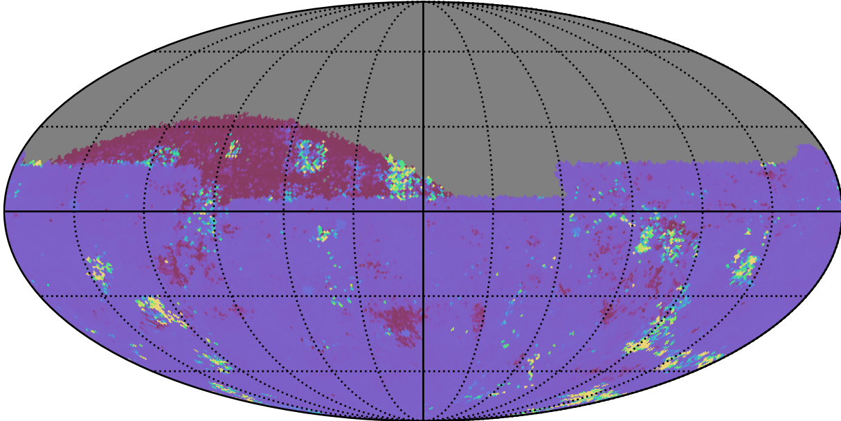
too_elab_heavy_r64_d3_gz_v3.4_10yrs All sky ug bands: 75th Percentile Intranight Timespan
