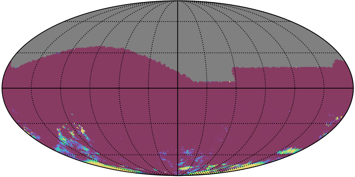
too_elab_heavy_r64_d3_gz_v3.4_10yrs All sky ri bands: 75th Percentile Intranight Timespan
