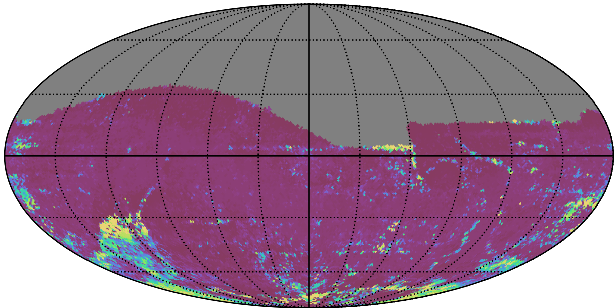
too_elab_heavy_r64_d3_gz_v3.4_10yrs All sky i band: 75th Percentile Intranight Timespan
