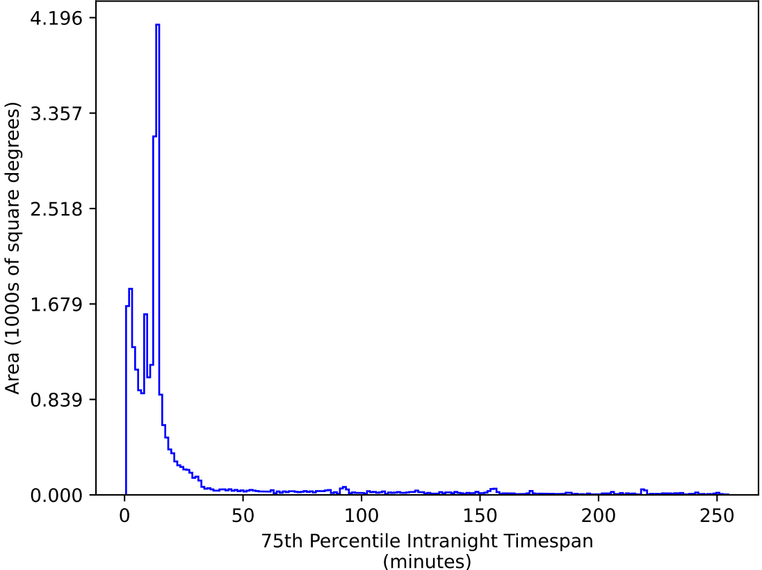
too_elab_heavy_r64_d3_gz_v3.4_10yrs All sky i band: 75th Percentile Intranight Timespan
