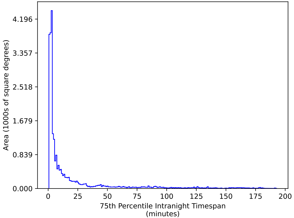
too_elab_heavy_r64_d3_gz_v3.4_10yrs All sky g band: 75th Percentile Intranight Timespan
