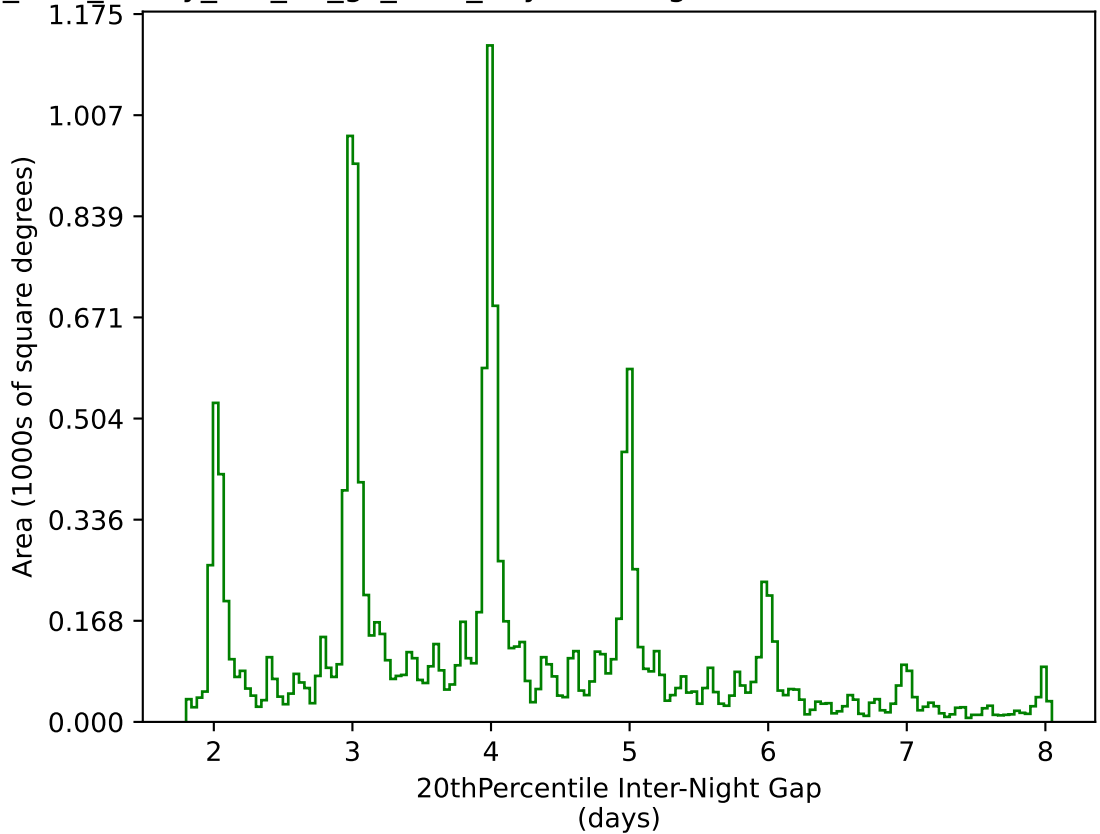
too_elab_heavy_r64_d3_gz_v3.4_10yrs WFD g band: 20thPercentile Inter-Night Gap
