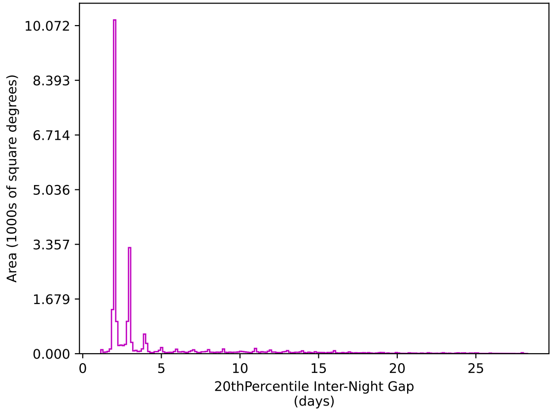
too_elab_heavy_r64_d3_gz_v3.4_10yrs All sky z band: 20thPercentile Inter-Night Gap
