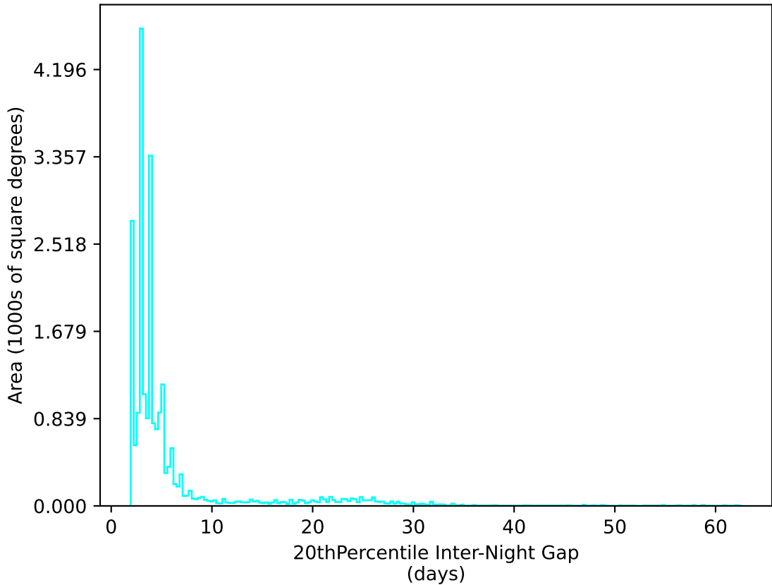
too_elab_heavy_r64_d3_gz_v3.4_10yrs All sky u band: 20thPercentile Inter-Night Gap
