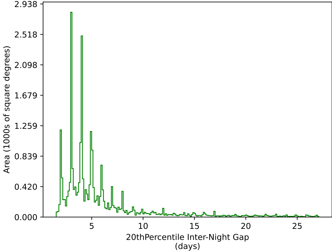
too_elab_heavy_r64_d3_gz_v3.4_10yrs All sky g band: 20thPercentile Inter-Night Gap
