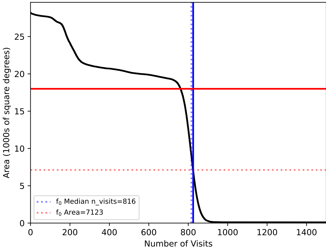
too_elab_heavy_r64_d3_gz_v3.4_10yrs : f0
