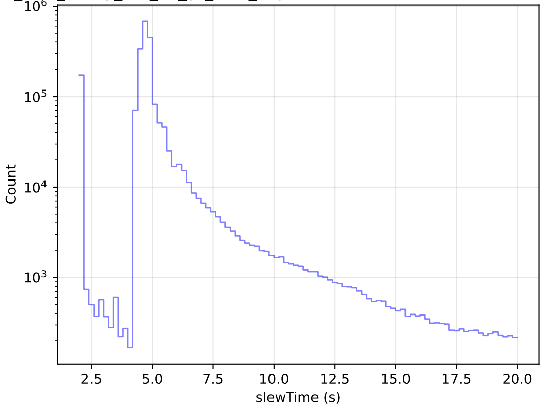
too_elab_heavy_r64_d3_gz_v3.4_10yrs All visits: Zoom Slew Time Histogram
