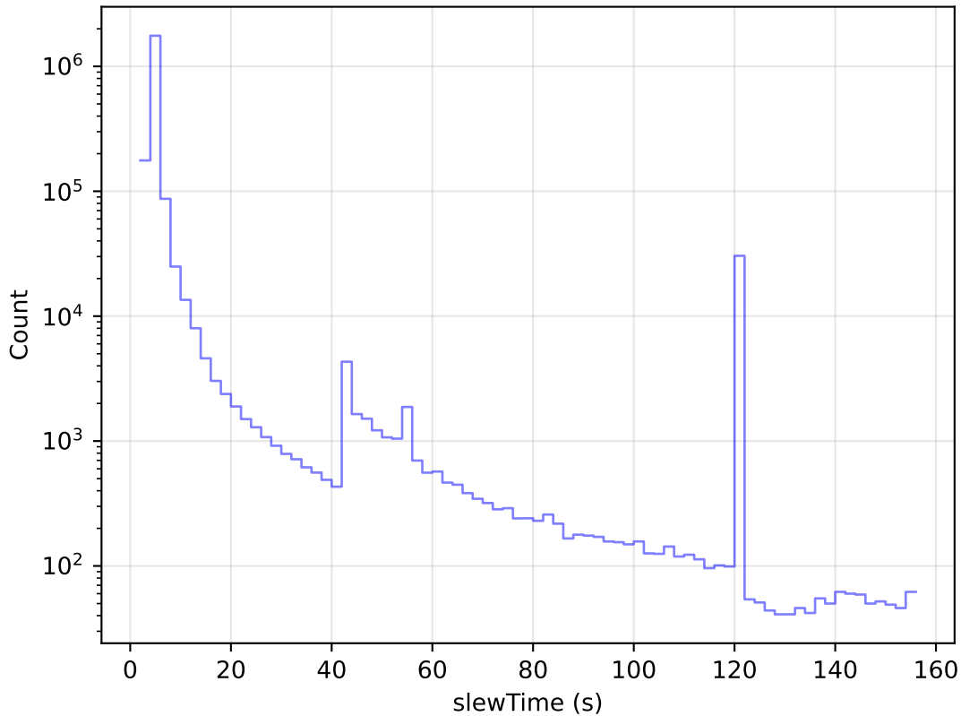
too_elab_heavy_r64_d3_gz_v3.4_10yrs All visits: Slew Time Histogram
