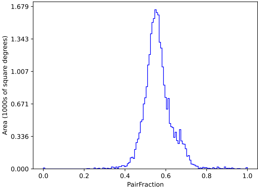
too_elab_heavy_r64_d3_gz_v3.4_10yrs (g or r or i): PairFraction
