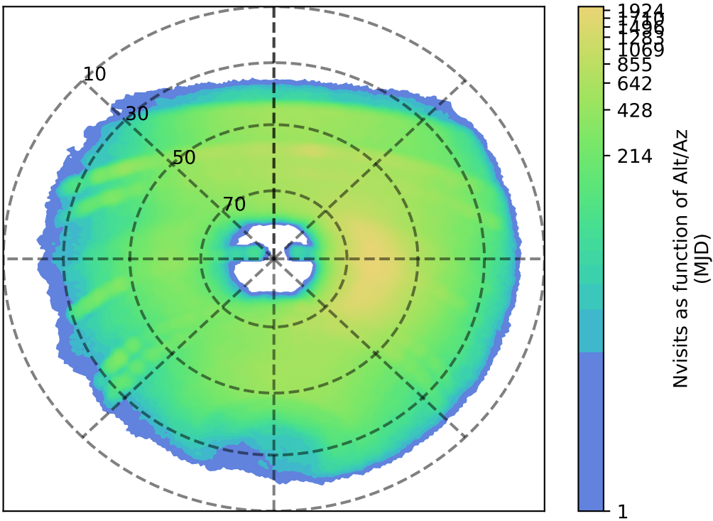
too_elab_heavy_r64_d3_gz_v3.4_10yrs y: Nvisits as function of Alt/Az
