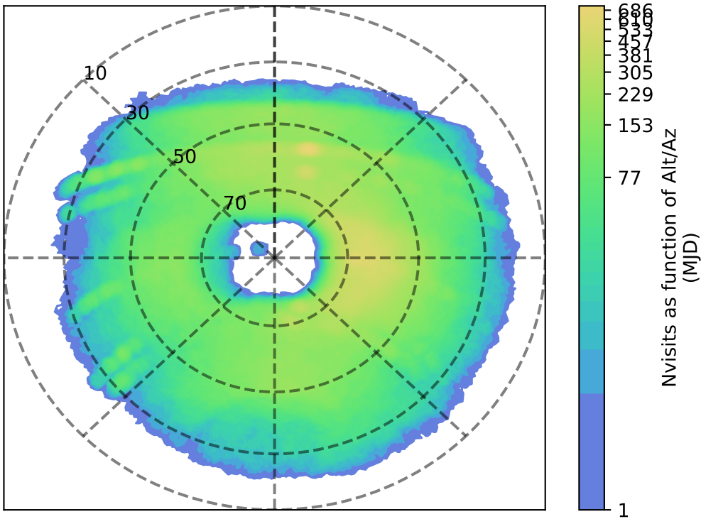
too_elab_heavy_r64_d3_gz_v3.4_10yrs u: Nvisits as function of Alt/Az
