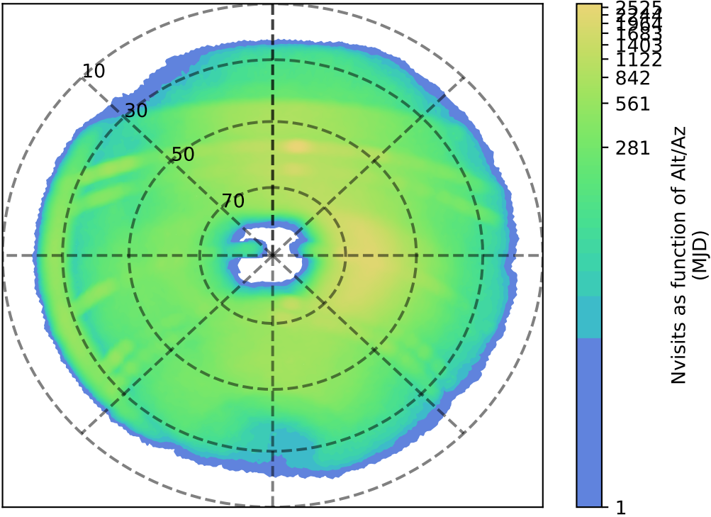
too_elab_heavy_r64_d3_gz_v3.4_10yrs r: Nvisits as function of Alt/Az
