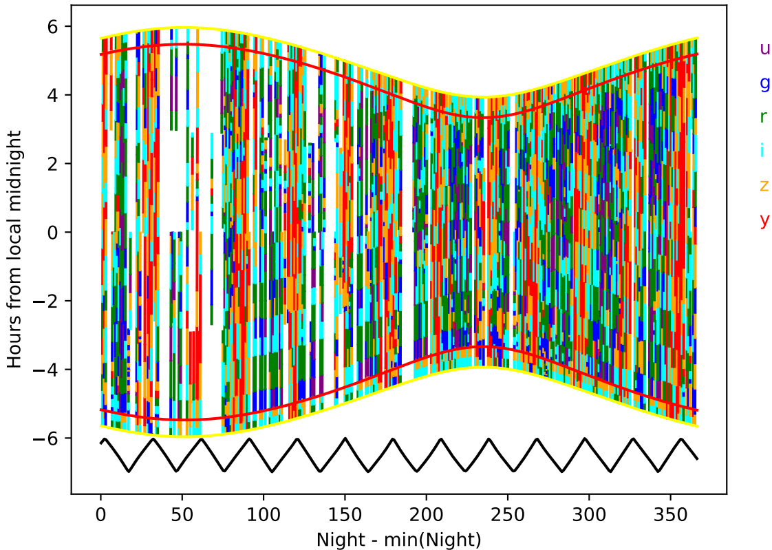
too_elab_heavy_r64_d3_gz_v3.4_10yrs year 9-10: Hourglass
