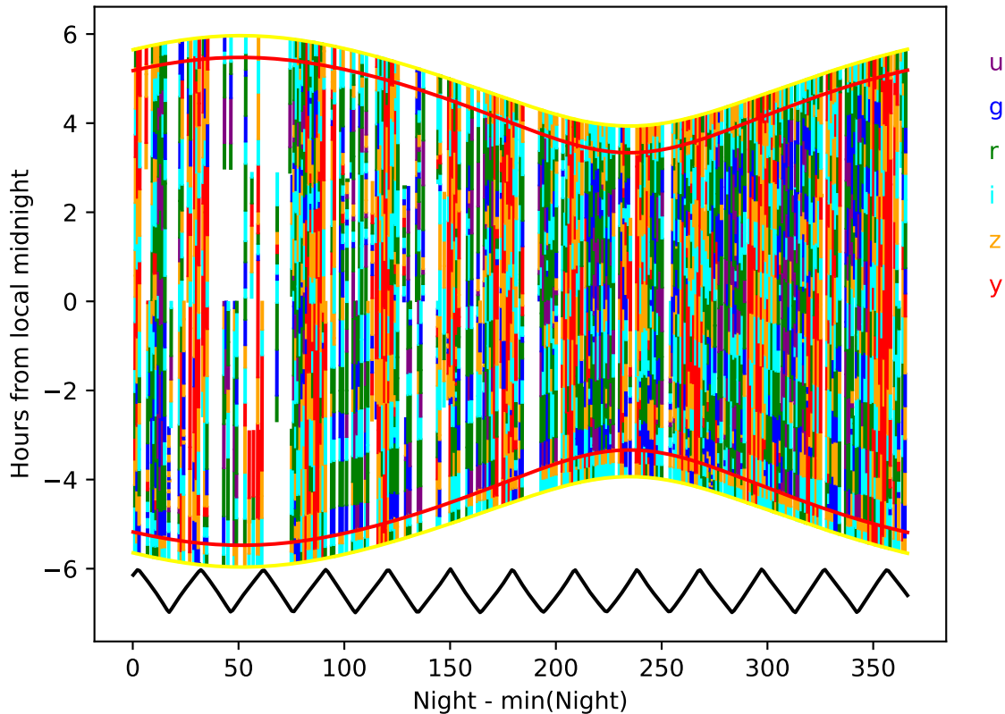
too_elab_heavy_r64_d3_gz_v3.4_10yrs year 9-10: Hourglass
