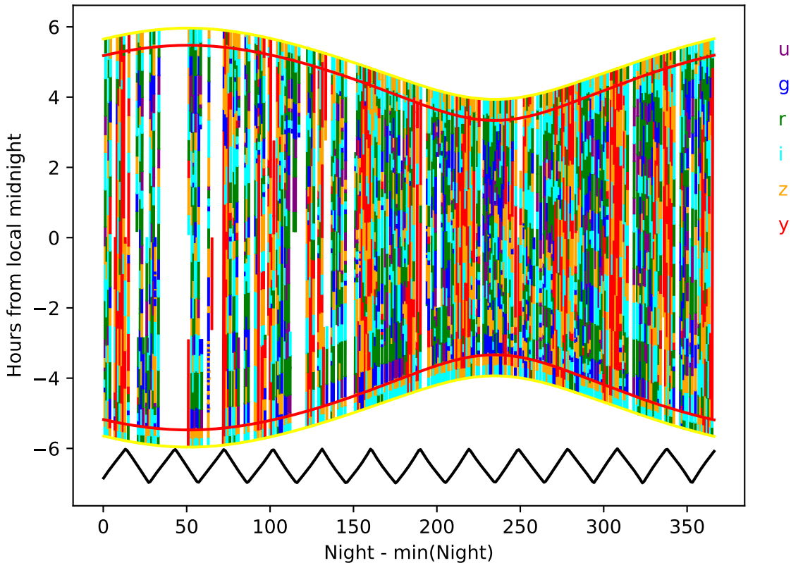
too_elab_heavy_r64_d3_gz_v3.4_10yrs year 8-9: Hourglass
