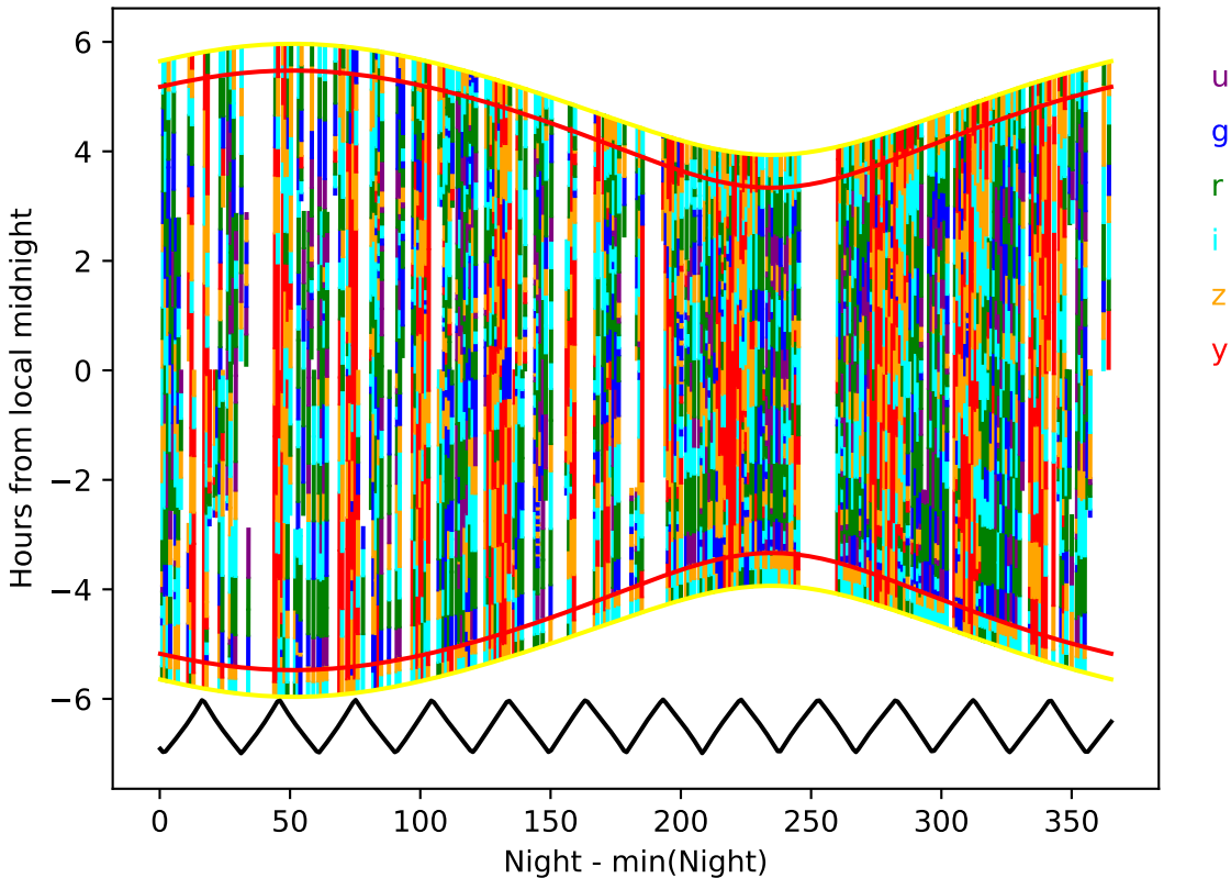
too_elab_heavy_r64_d3_gz_v3.4_10yrs year 5-6: Hourglass
