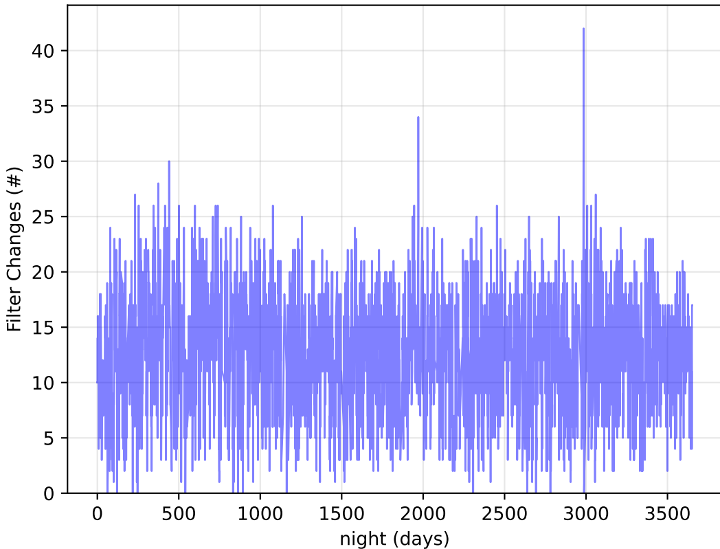
too_elab_heavy_r64_d3_gz_v3.4_10yrs : Filter Changes
