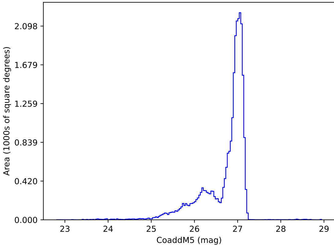
too_elab_heavy_r64_d3_gz_v3.4_10yrs r: CoaddM5
