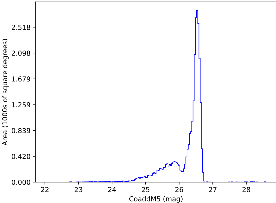
too_elab_heavy_r64_d3_gz_v3.4_10yrs i: CoaddM5
