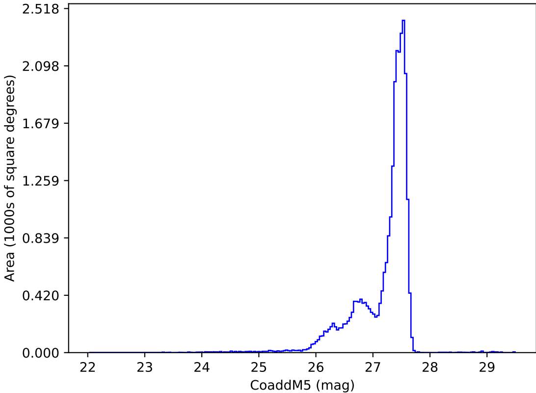
too_elab_heavy_r64_d3_gz_v3.4_10yrs : CoaddM5
