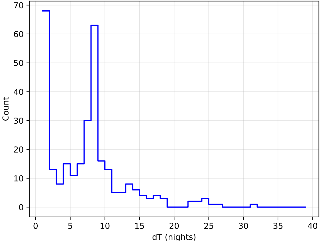
too_elab_heavy_r64_d3_gz_v3.4_10yrs all bands: DD:XMM_LSS Delta Nights Histogram
