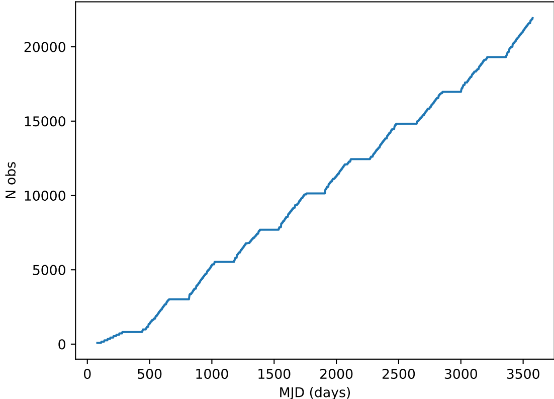
too_elab_heavy_r64_d3_gz_v3.4_10yrs all bands: DD:XMM_LSS Cumulative NVisits
