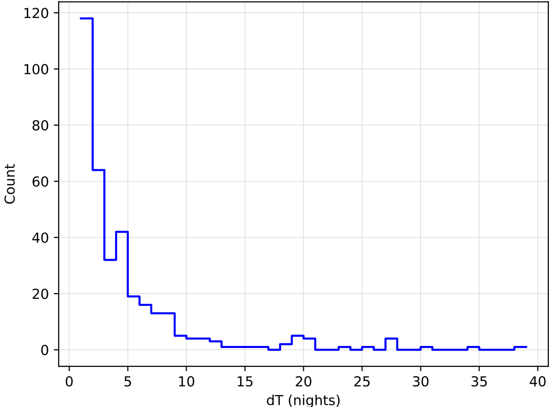
too_elab_heavy_r64_d3_gz_v3.4_10yrs all bands: DD:WFD Delta Nights Histogram
