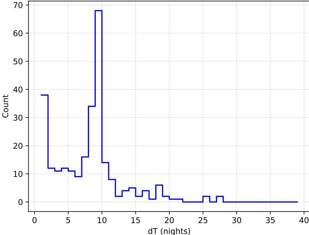
too_elab_heavy_r64_d3_gz_v3.4_10yrs all bands: DD:ELAISS1 Delta Nights Histogram
