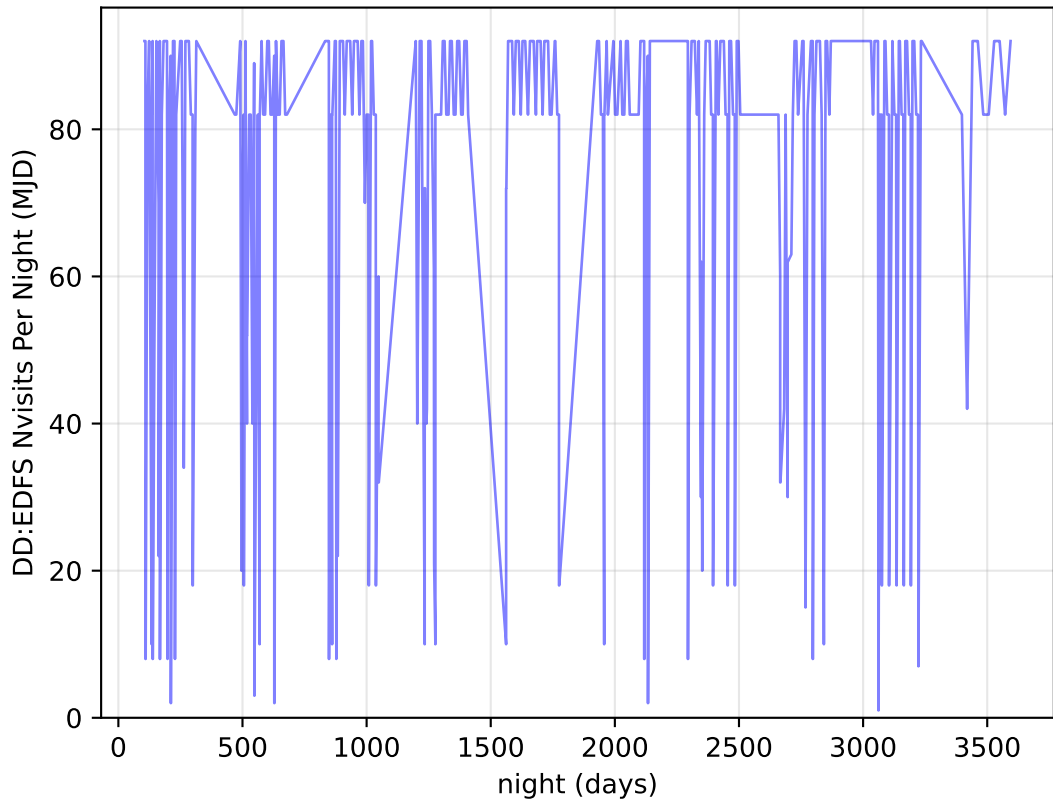
too_elab_heavy_r64_d3_gz_v3.4_10yrs all bands: DD:EDFS Nvisits Per Night
