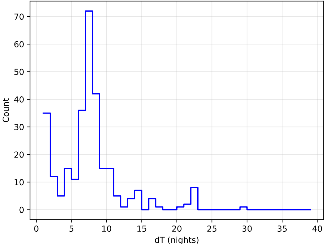
too_elab_heavy_r64_d3_gz_v3.4_10yrs all bands: DD:EDFS Delta Nights Histogram
