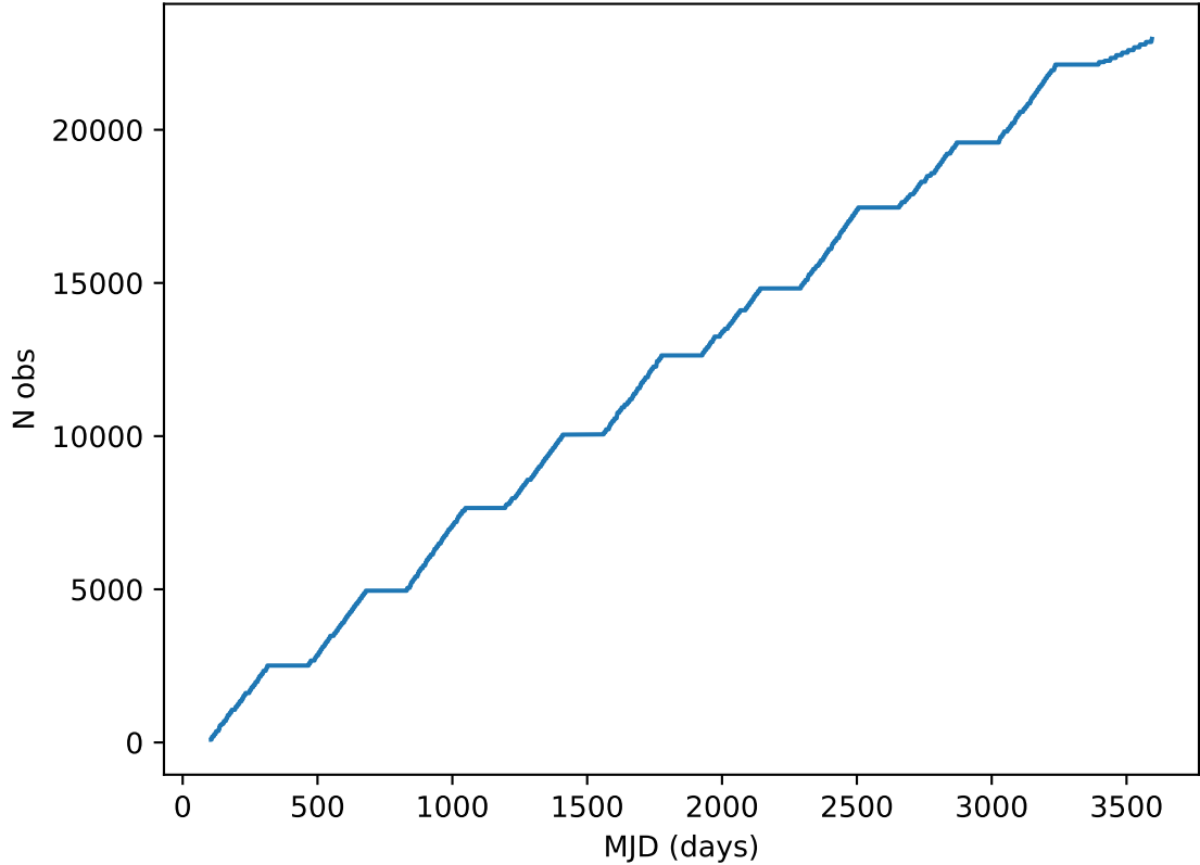
too_elab_heavy_r64_d3_gz_v3.4_10yrs all bands: DD:EDFS Cumulative NVisits
