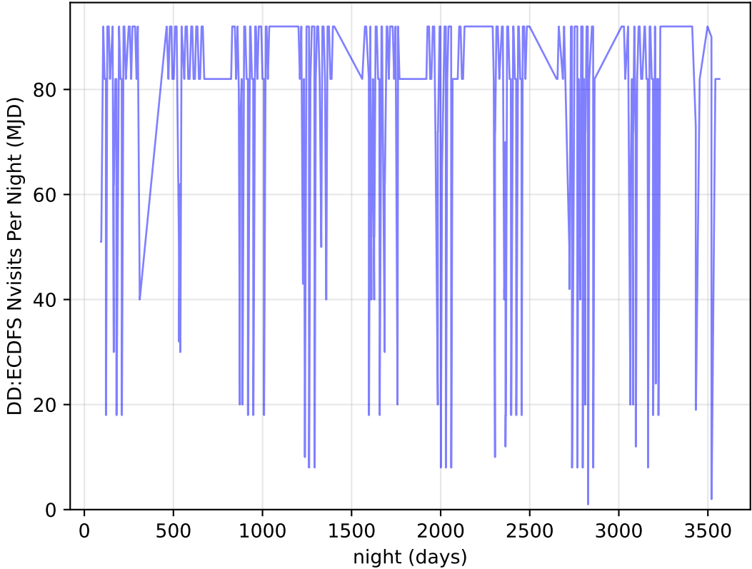
too_elab_heavy_r64_d3_gz_v3.4_10yrs all bands: DD:ECDFS Nvisits Per Night
