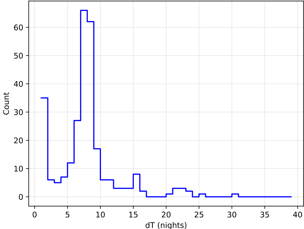
too_elab_heavy_r64_d3_gz_v3.4_10yrs all bands: DD:ECDFS Delta Nights Histogram
